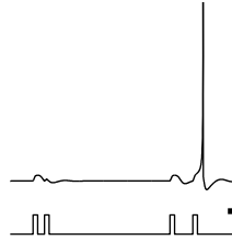
(K) resonator
