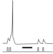
(L) integrator
