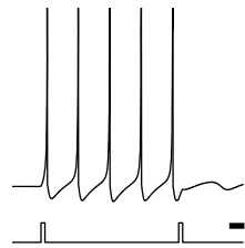
(P) bistability
