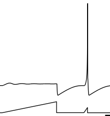
(R) accommodation
